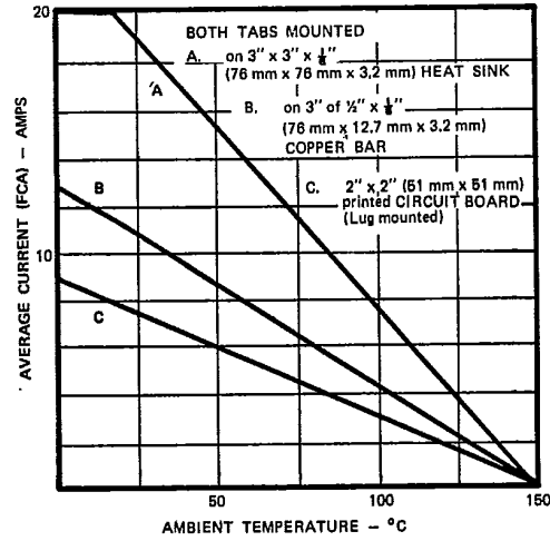
Fig. 2 - Forward Current Vs. Ambient Temperature
