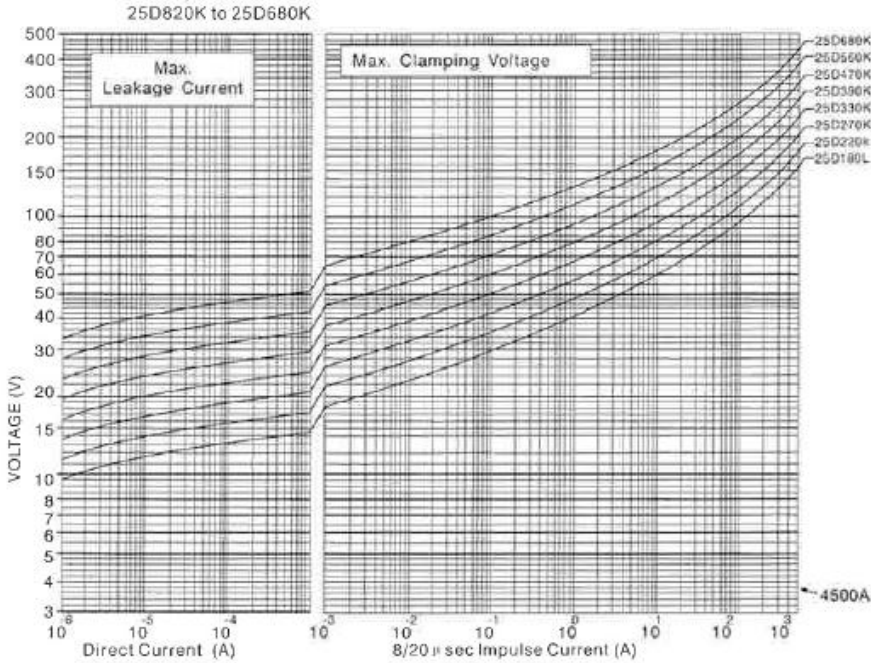
V-I curve
