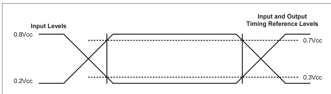
Figure 46, AC Measurement I/O Waveform
