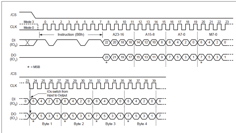
Figure 17, Dual I/O Fast Read Sequence Diagram (M5-4 \neq (1, 0))
