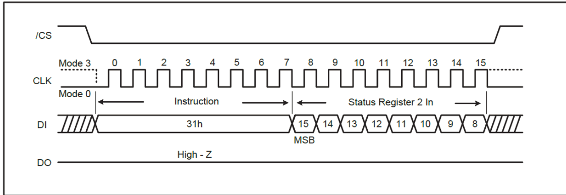
Figure 12a. Write Status Register-2 Instruction
