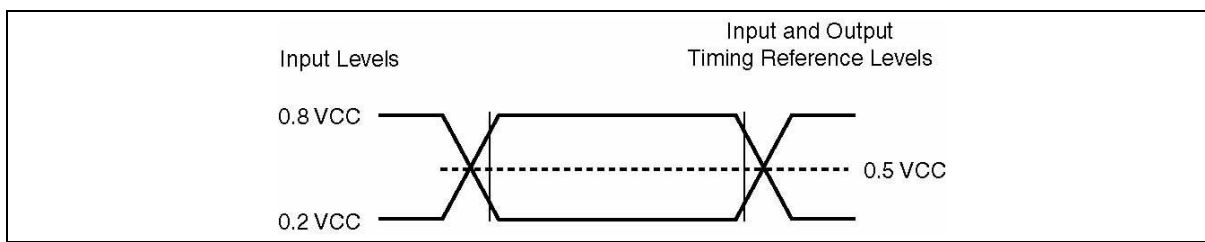
Figure 38. AC Measurement I/O Waveform
