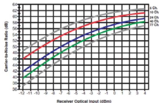
Carrier-to-Noise Performance
