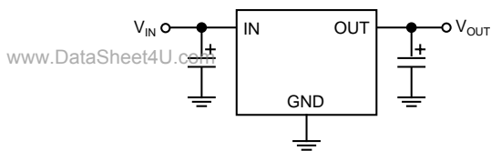
Figure 3. Linear regulators require only two capacitors for operation.
