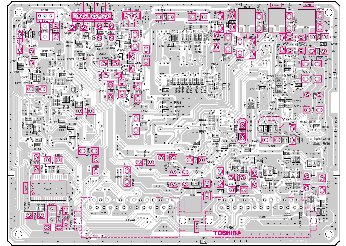
DIGITAL BOARD PD2215-1 BOTTOM (FOIL) SIDE
