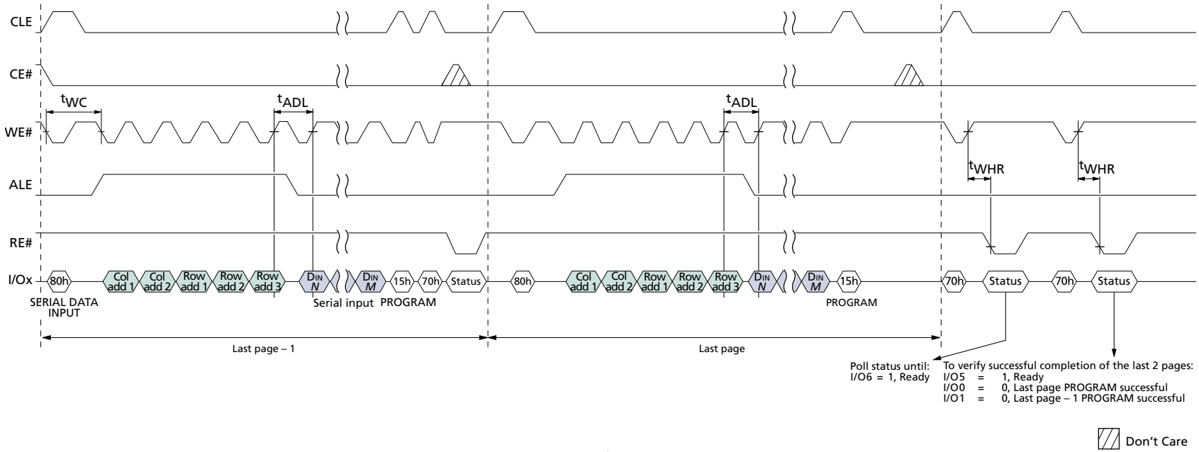
Figure 90: PROGRAM PAGE CACHE MODE Operation Ending on 15h
