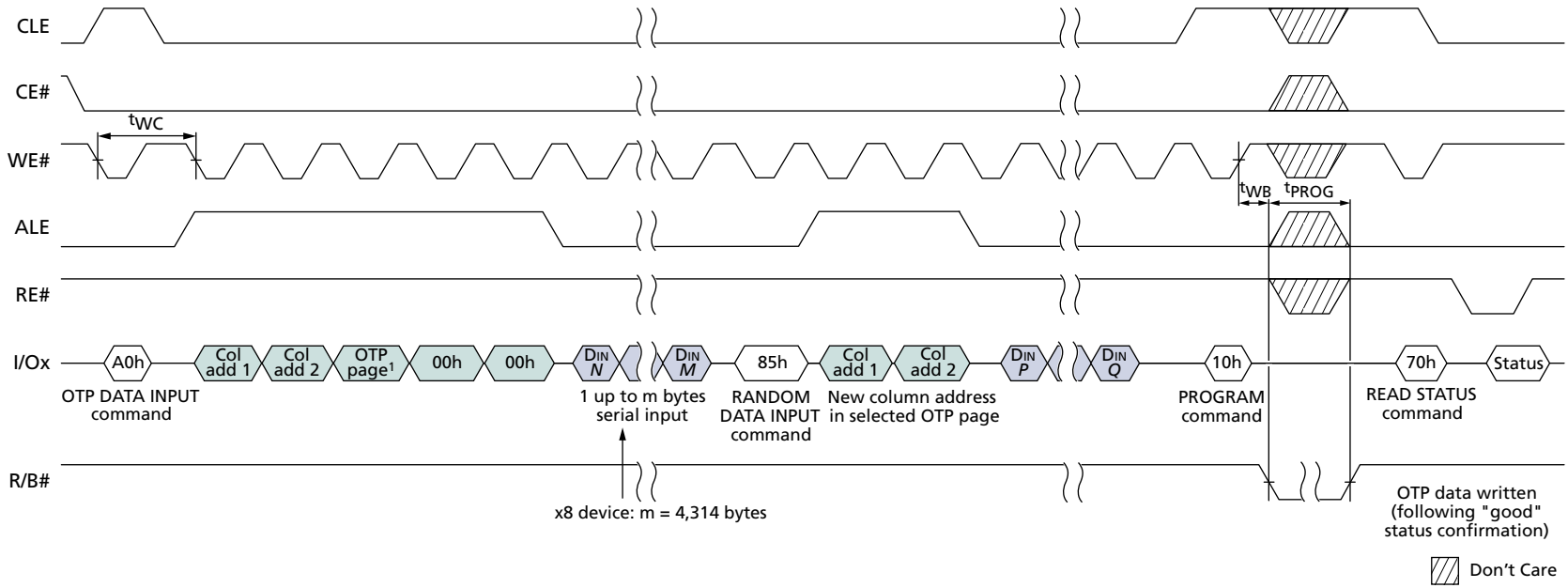
Figure 28: OTP PROGRAM with RANDOM DATA INPUT
