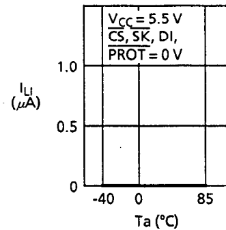
1.13 Input leakage current I_{LI} - Ambient temperature T_a
