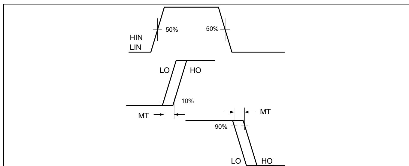
Figure 9 Delay matching waveform definition
