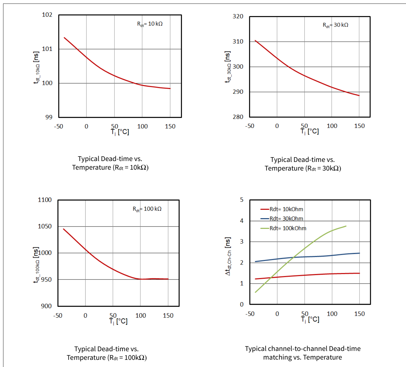
Figure 20 Typical Dead-time
