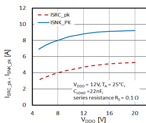
Typical peak output current vs. supply voltage
