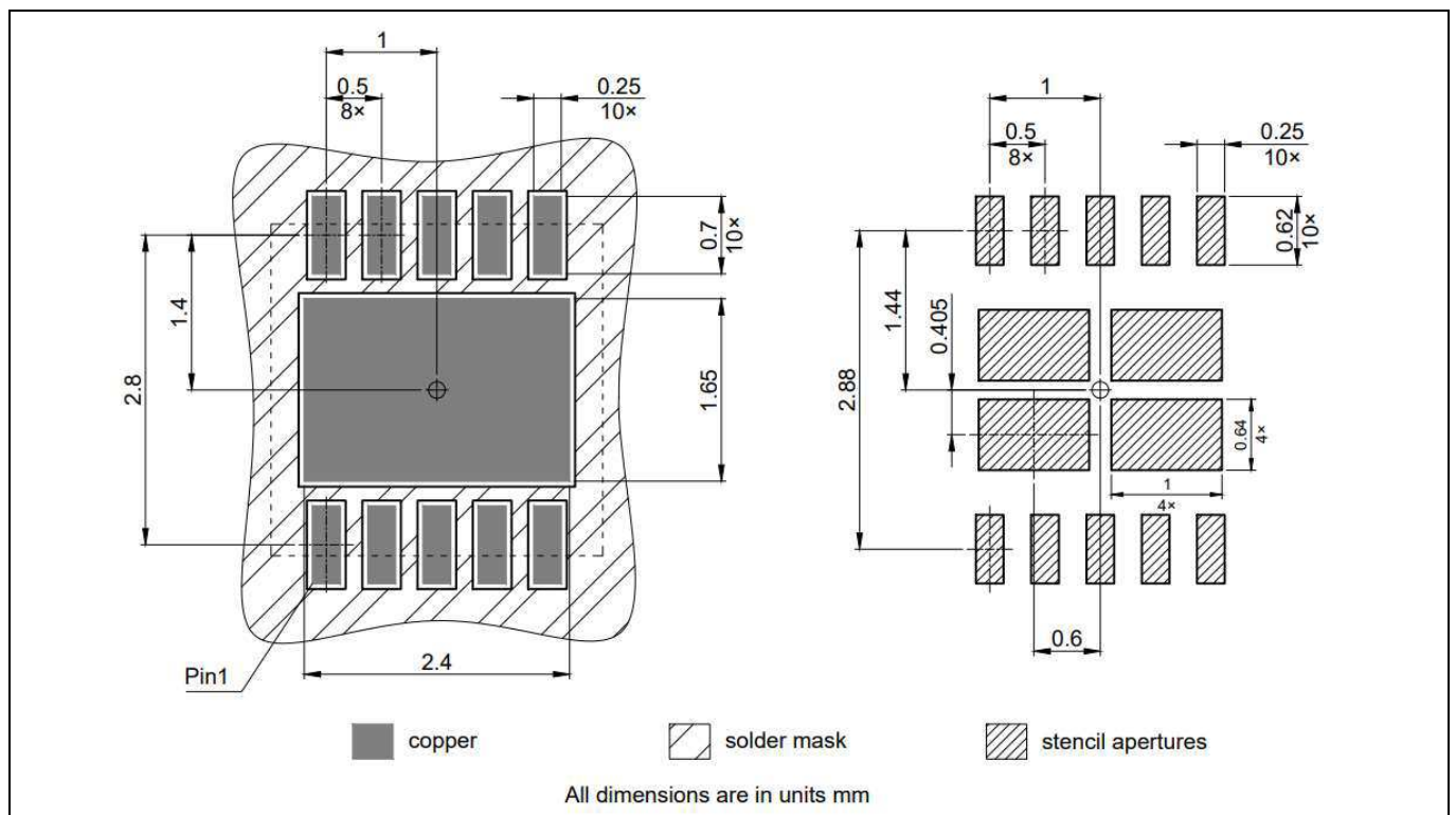
Figure 17 PG-VSON-10-4 Footprint Dimensions
