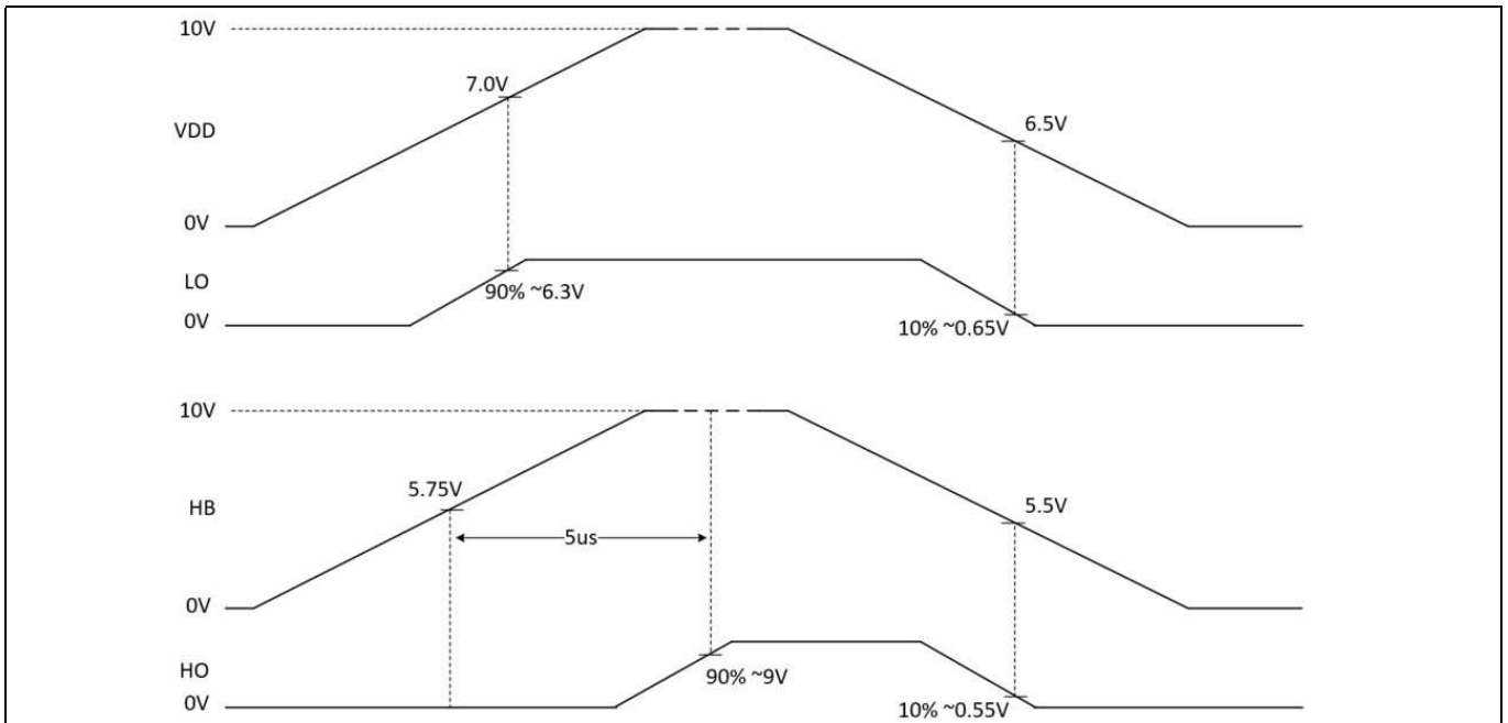
Figure 7 UVLO behavior
