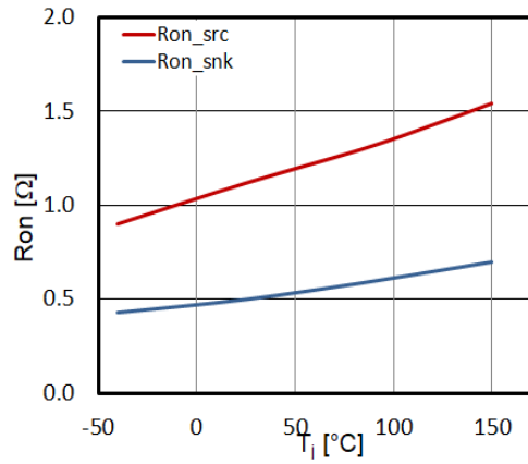
Typical output resistance vs. temperature
