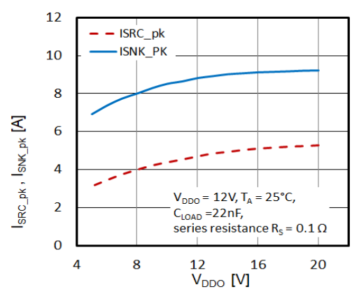
Typical peak output current vs. supply voltage
