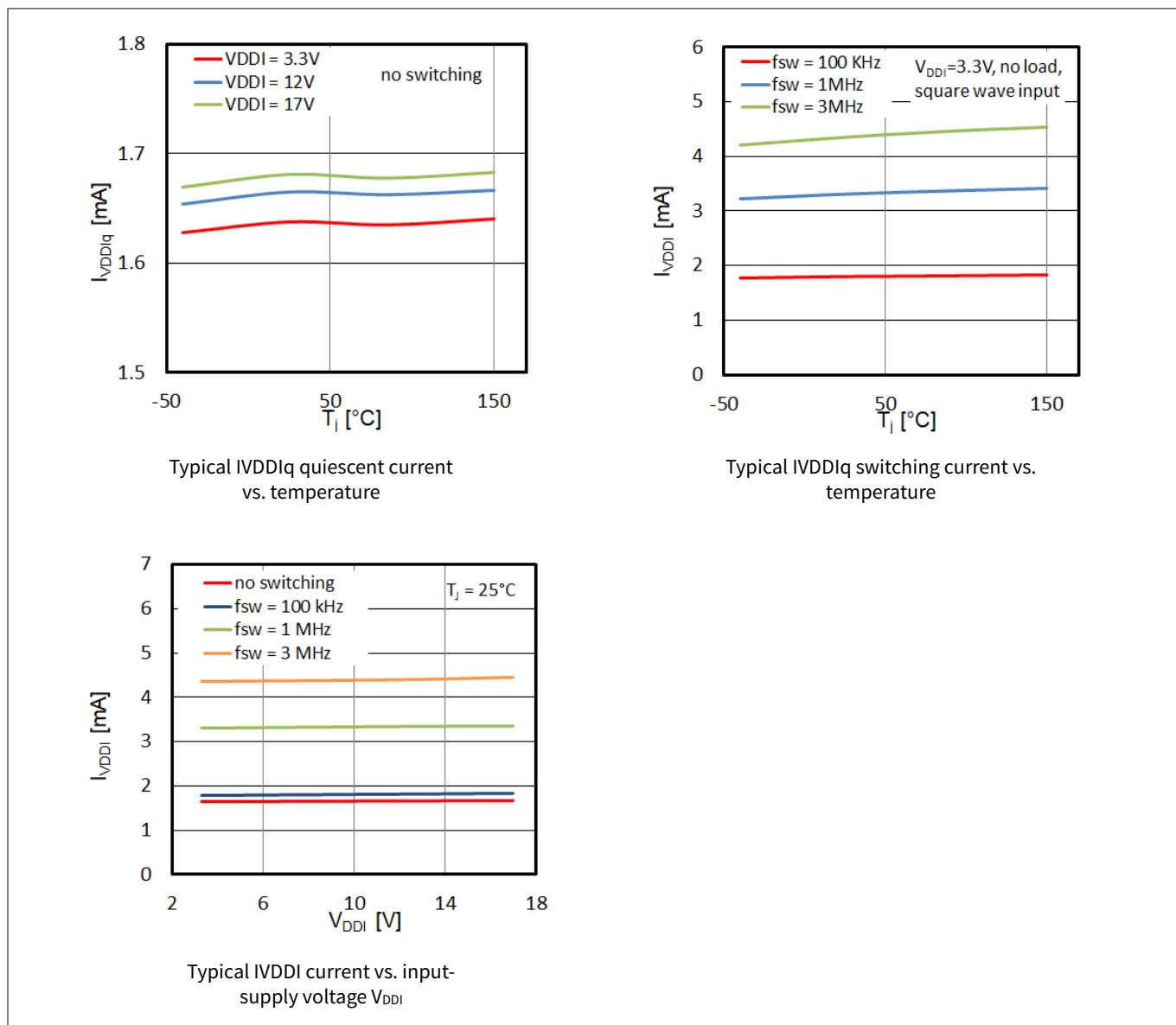
Figure 15 Input-side supply current
