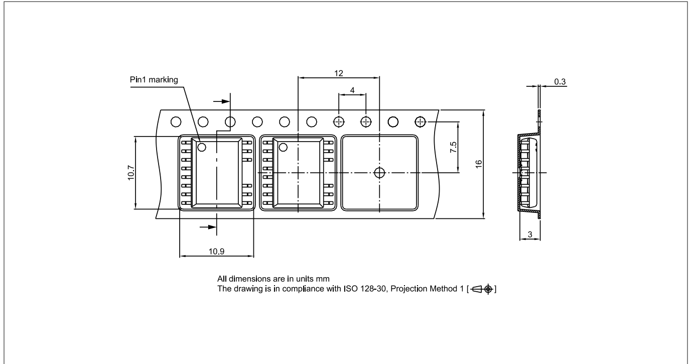
Figure 26 DSO14-300mil packing
