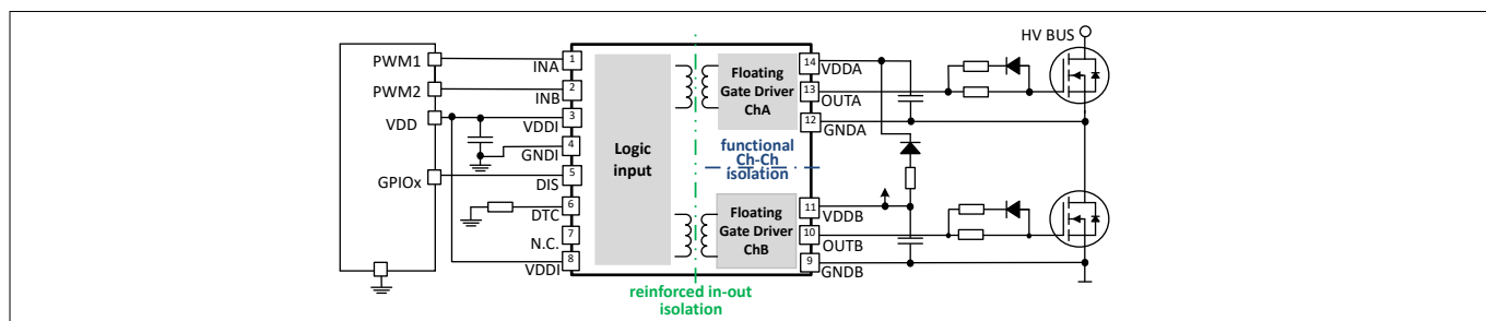
Figure 1 Application diagram
