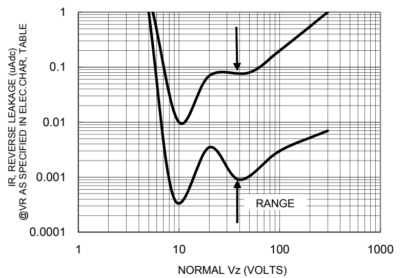
FIG. 3- TYPICAL REVERSE LEAKAGE
