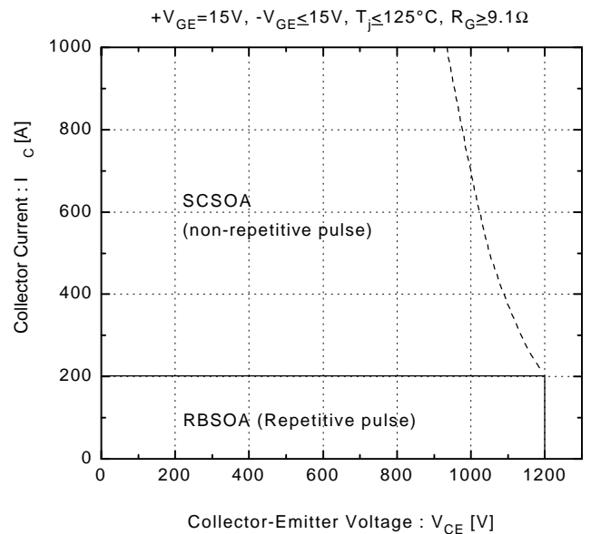
Reversed Biased Safe Operating Area
