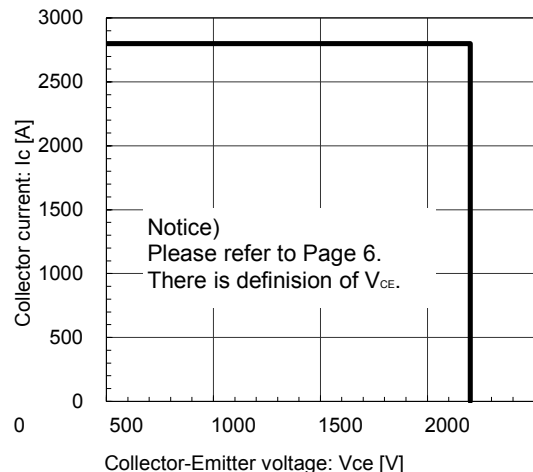
Reverse bias safe operating area (max.)
