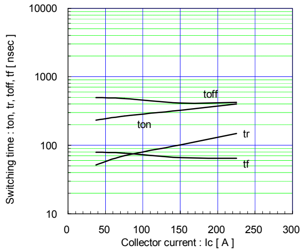
Switching time vs. Collector current (typ.) Vcc=600V, VGE=±15V, RG=4.7Ω, Tj=25°C
