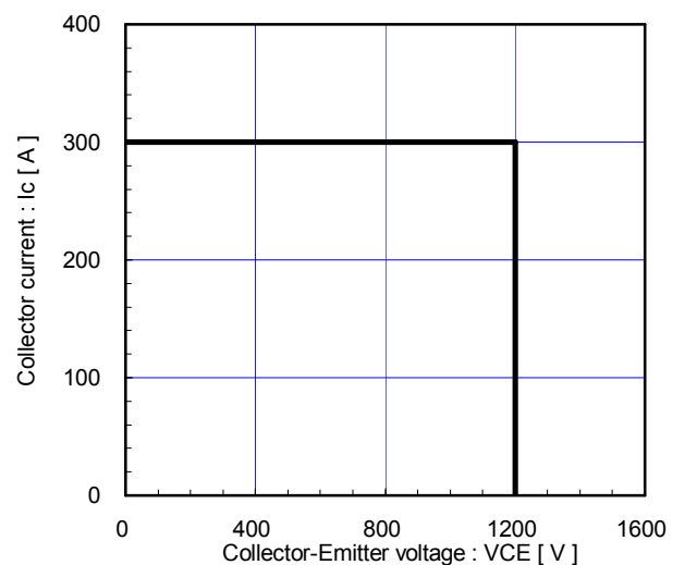
Reverse bias safe operating area (max.) +VGE=15V, -VGE ≤ 15V, RG ≥ 4.7Ω, Tj ≤ 125°C
