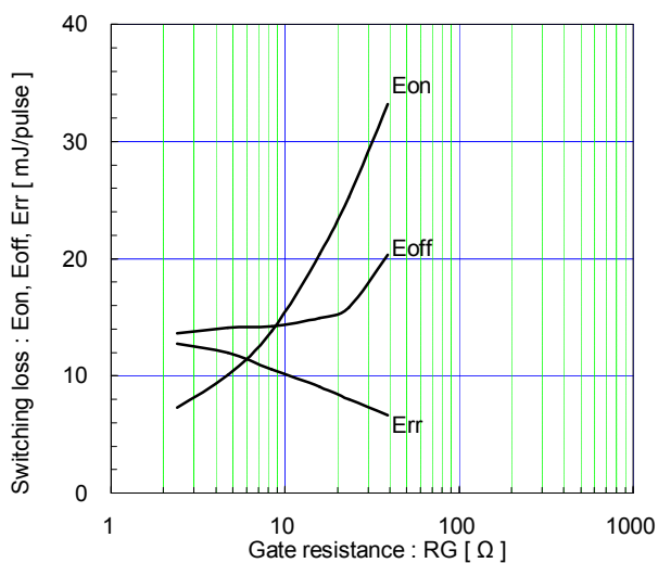
Switching loss vs. Gate resistance (typ.) Vcc=600V, Ic=150A, VGE=±15V, Tj=125°C
