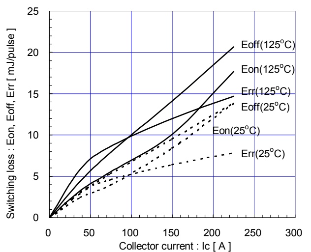
Switching loss vs. Collector current (typ.) Vcc=600V, VGE=±15V, RG=4.7Ω
