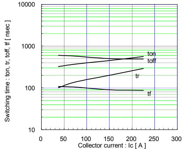
Switching time vs. Collector current (typ.) Vcc=600V, VGE=±15V, RG=4.7Ω, Tj=125°C
