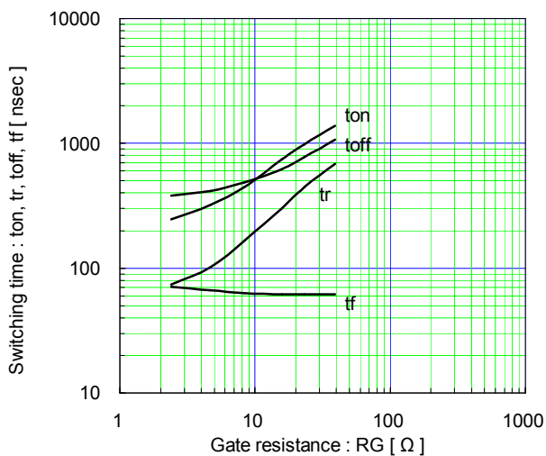
Switching time vs. Gate resistance (typ.) Vcc=600V, Ic=150A, VGE=±15V, Tj=25°C
