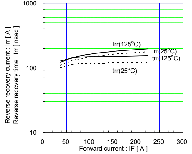
Reverse recovery characteristics (typ.) Vcc=600V, VGE=±15V, RG=4.7Ω
