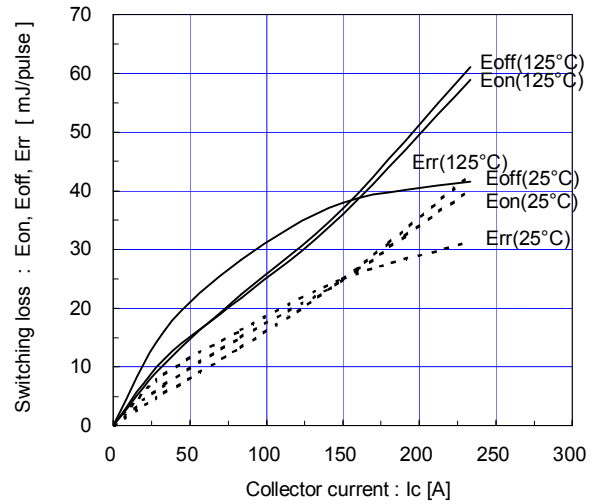
Switching loss vs. Collector current (typ.) V_{cc}=900V, V_{GE}=\pm 15V, R_g=3.3\Omega
