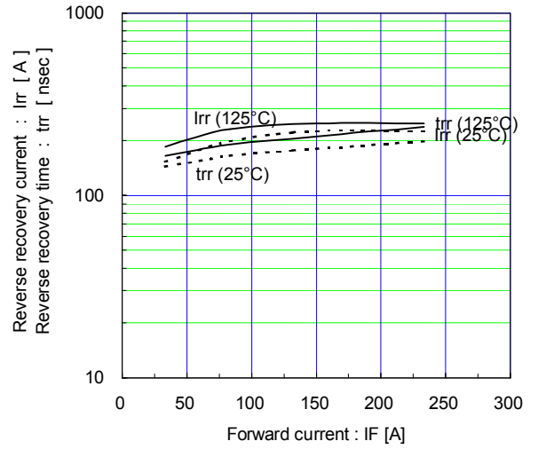
Reverse recovery characteristics (typ.) Vcc=900V, VGE=±15V, Rg=3.3Ω
