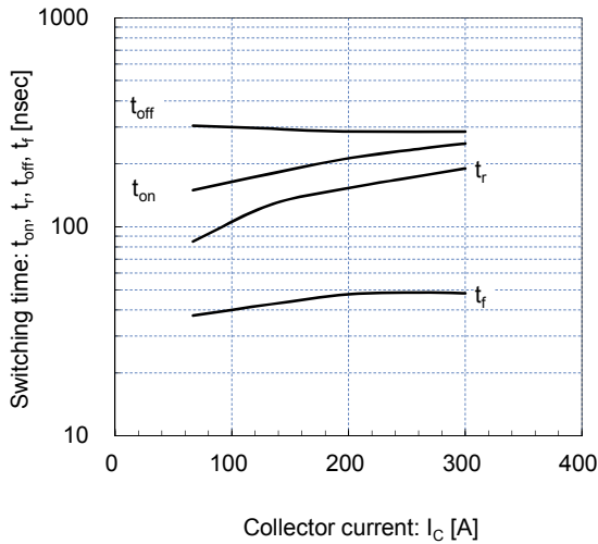
Switching time vs. Collector current (typ.) V cc =600V, V GE =±15V, R g =4.7Ω, T j =25°C
