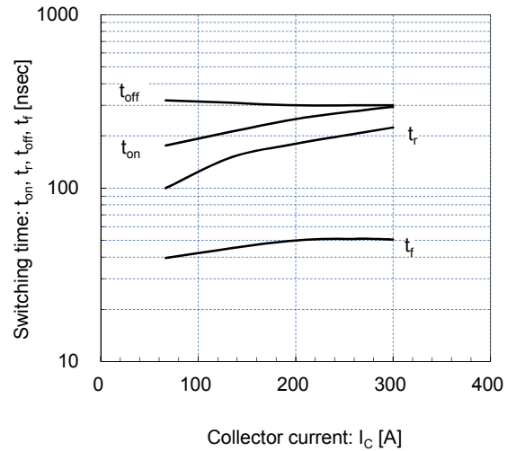
Switching time vs. Collector current (typ.) V cc =600V, V GE =±15V, R g =4.7Ω, T j =125°C
