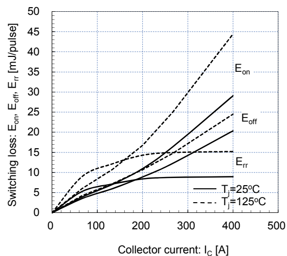
Switching loss vs. Collector current (typ.) V cc =600V, V GE =±15V, R g =4.7Ω, T j =25, 125°C
