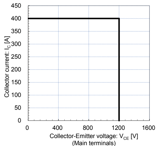
Reverse bias safe operating area (max.) +V GE =15V, -V GE =15V, R g =4.7Ω, T j =125°C
