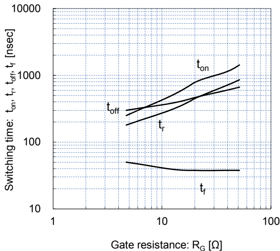
Switching time vs. Gate resistance (typ.) V cc =600V, I c =200A, V GE =±15V, T j =125°C
