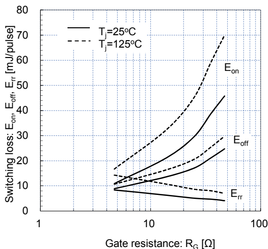
Switching loss vs. Gate resistance (typ.) V cc =600V, I c =200A, V GE =±15V, T j =25, 125°C
