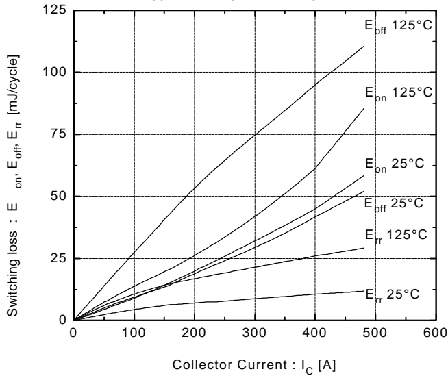
Switching loss vs. Collector current V_{CC}=600V, R_{GE}=2.7\Omega, V_{GE}=\pm 15V
