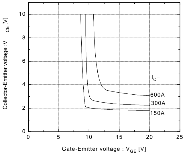
Collector-Emmitter vs. Gate-Emmitter voltage T_j=25^\circ\text{C}
