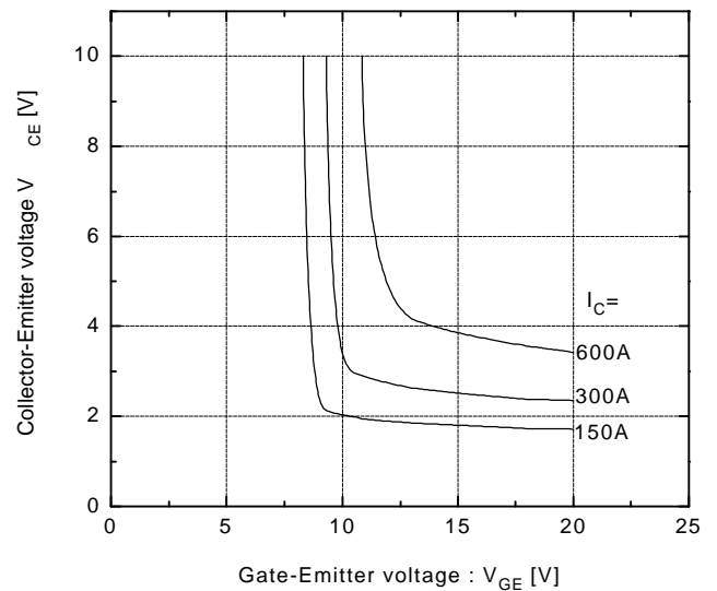
Collector-Emmitter vs. Gate-Emmitter voltage T_j=125^\circ\text{C}
