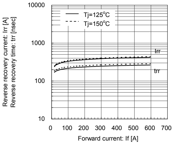
Reverse Recovery Characteristics (typ.) V_{cc}=600\text{V} , V_{ge}=\pm 15\text{V} , R_g=0.93\Omega , T_j=125^\circ\text{C} , 150^\circ\text{C}
