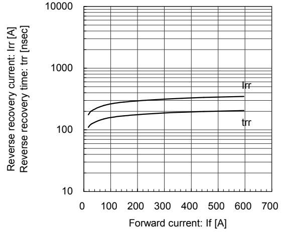
Reverse Recovery Characteristics (typ.) V_{cc}=600\text{V} , V_{ge}=\pm 15\text{V} , R_g=0.93\Omega , T_j=25^\circ\text{C}
