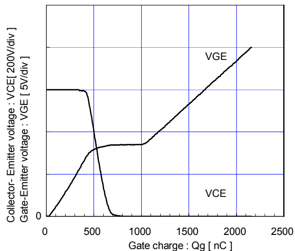
Dynamic Gate charge (typ.) Vcc=600V, Ic=450A, Tj=25°C
