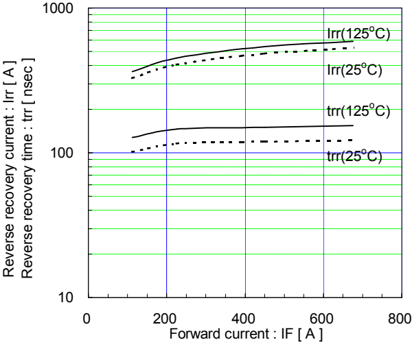
Reverse recovery characteristics (typ.) Vcc=600V, VGE=±15V, RG=1.1Ω
