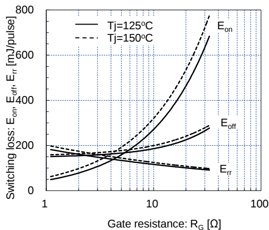
Switching loss vs. Gate resistance (typ.) V cc =900V, I c =550A, V GE =±15V, T j =125°C, 150°C
