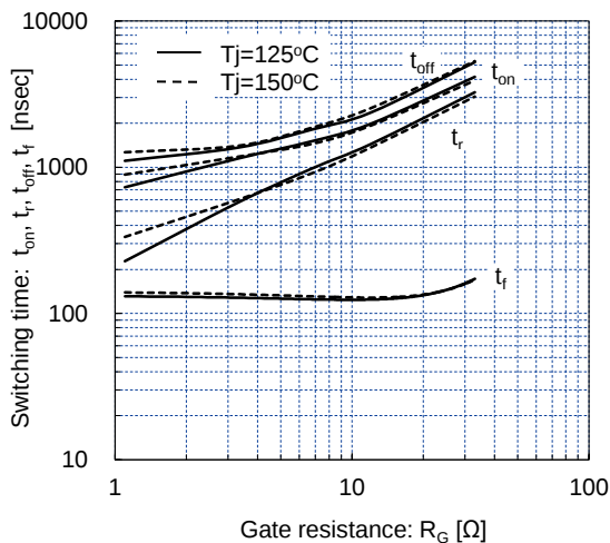
Switching time vs. Gate resistance (typ.) V cc =900V, I c =550A, V GE =±15V, T j =125°C, 150°C
