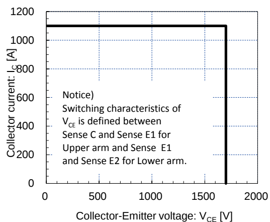
Reverse bias safe operating area (max.) +V GE =15V, -V GE =15V, R g =3.3Ω, T j =150°C
