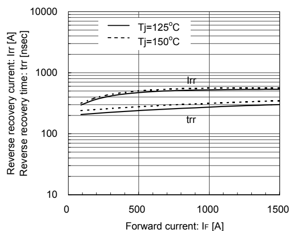
Reverse Recovery Characteristics (typ.) V_{CC}=600\text{V} , V_{GE}=\pm 15\text{V} , R_G=1.6\Omega , T_j=125^\circ\text{C} , 150^\circ\text{C}
