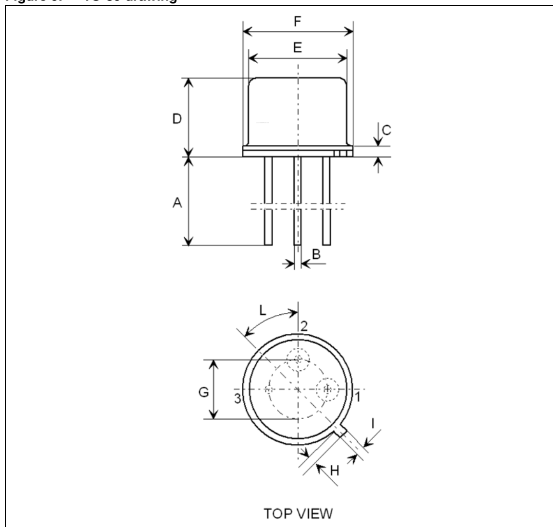
Figure 9. TO-39 drawing
