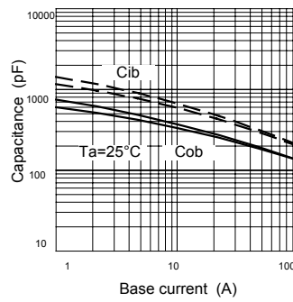
Figure 10 Capacitances
