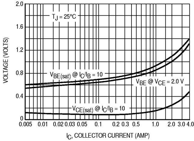
Figure 3. "On" Voltage
