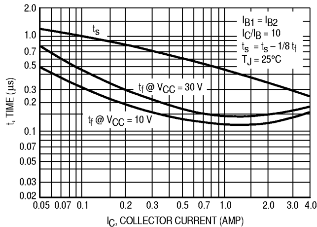
Figure 10. Turn-Off Time
