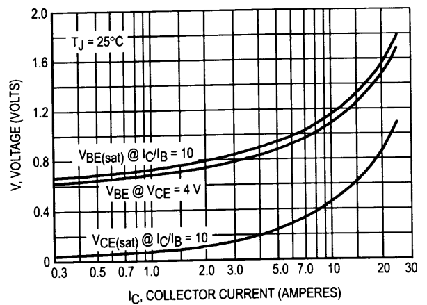
Figure 10. "On" Voltages
