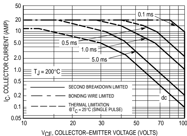
Figure 6. 2N6052, 2N6059
