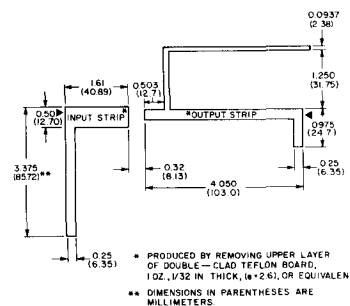
Fig. 10—400-MHz amplifier test circuit for measurement of output power for both types.
