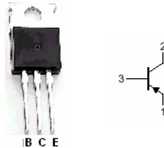
Fig.1 simplified outline (TO-220) and symbol
