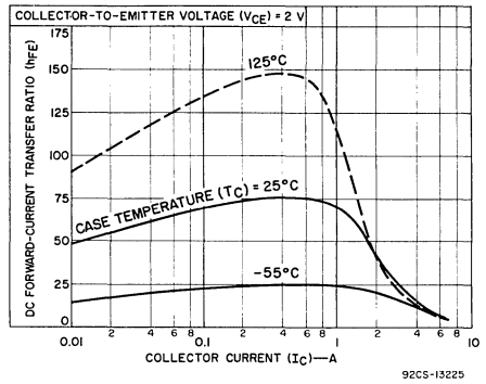
Fig. 12 - Typical dc beta characteristics for 2N3878, 2N3879, and 40375.
