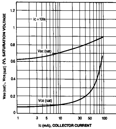
COLLECTOR EMITTER SATURATION VOLTAGE BASE EMITTER SATURATION VOLTAGE
