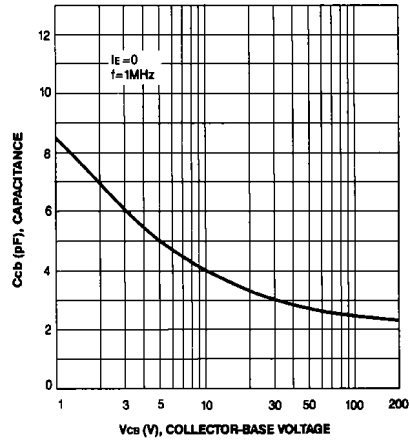
COLLECTOR-BASE CAPACITANCE
