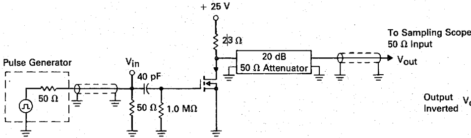
FIGURE 1 — SWITCHING TEST CIRCUIT
