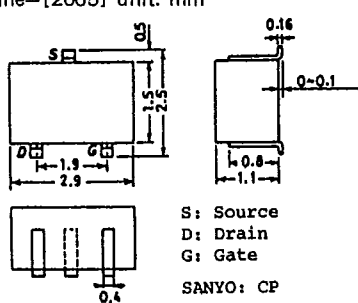
Case Outline—[2065] unit: mm
