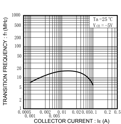
Fig.7 TRANSITION FREQUENCY vs. EMITTER CURRENT
