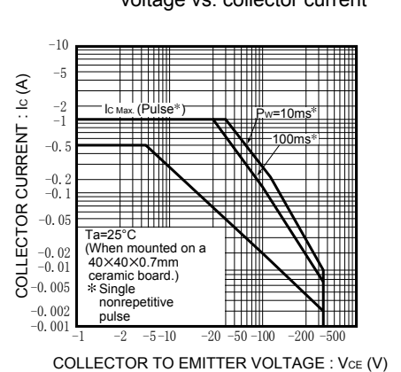
Fig.9 Safe operating area (2SA1812)
