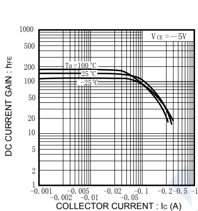
Fig.4 DC current gain vs. collector current (II)
