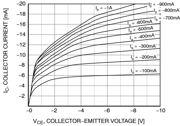
Figure 1. Static Characteristic
