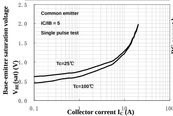
Saturation Voltage
