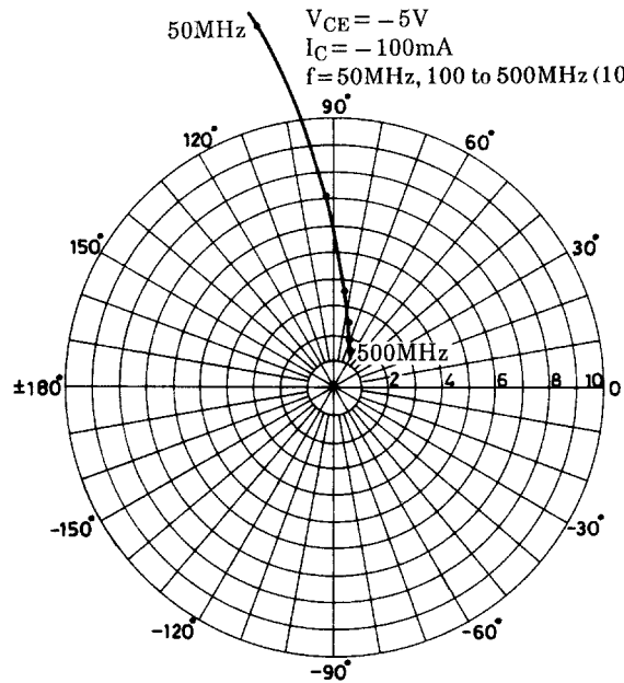
2SA1969 S21e
