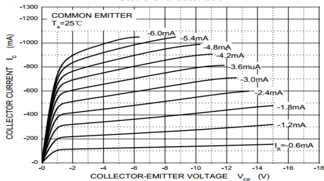
Static Characteristic
