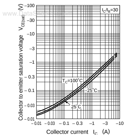
V_{CE(\text{sat})} - I_C
