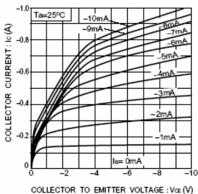
Fig.1 Ground emitter output characteristics
