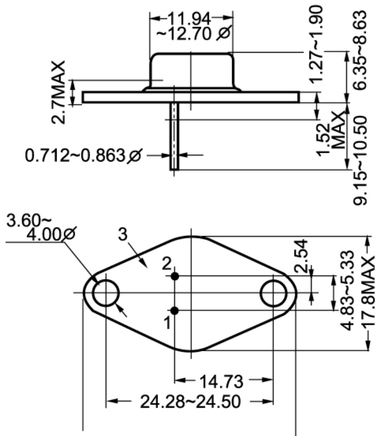
Fig.2 Outline dimensions
