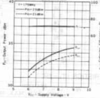
OUTPUT POWER & COLLECTOR EFFICIENCY vs. SUPPLY VOLTAGE
