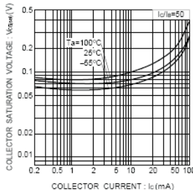
Fig.8 Collector-Emitter Saturation Voltage vs. Collector Current
