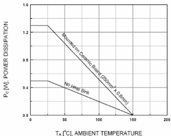
Figure 8. Power Derating
