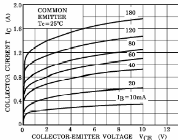
Fig.3 Static Characteristic
