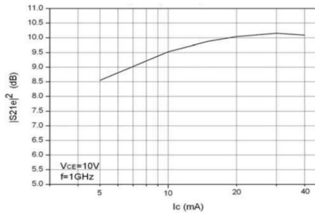
Fig 4. |S_{21e}|^2 vs. I_c
