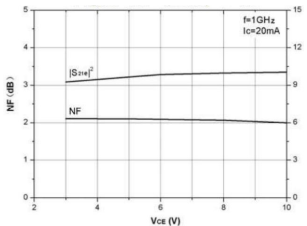
Fig 6. |S_{21e}|^2 vs. V_{CE}
